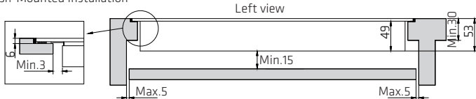
Flush-Mounted Installation
