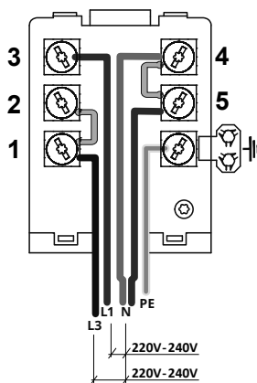
380-415V ~ 2+N+GND
