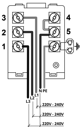
380-415V ~ 3+N+GND
